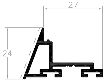
L53843 remate inferior
