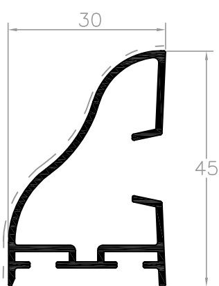
L50812 pingadeira decorativa
