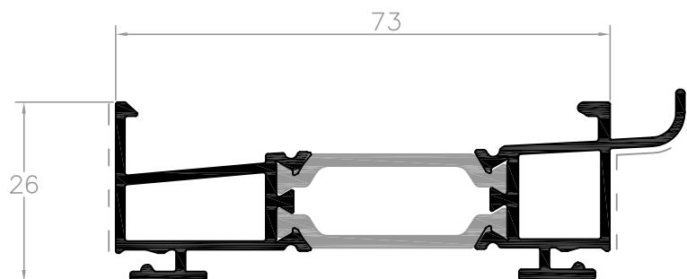
L58702 soleira c/ remate
