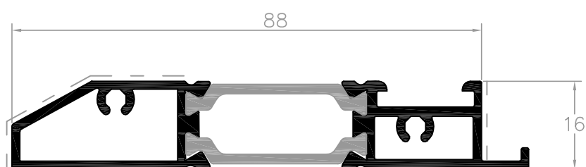
L57814 remate soleira
