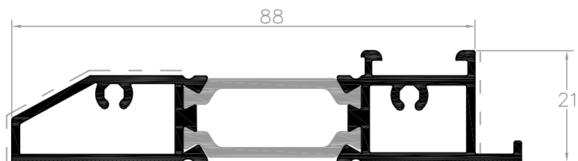
L57813 remate soleira
