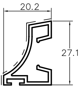
L50808 pingadeira
