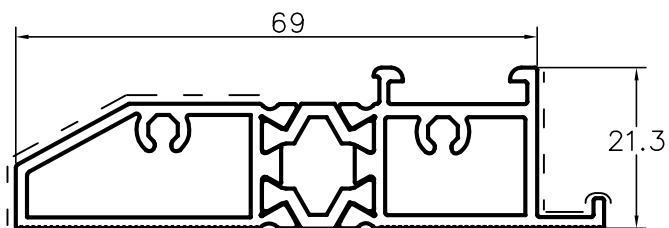
L53813 remate soleira
