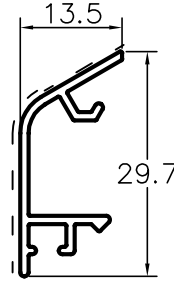
L50806 pingadeira
