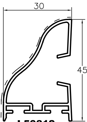
L50812 pingadeira decorativa
