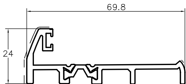
L53812 remate soleira
