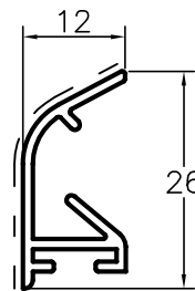
L50816 pingadeira
