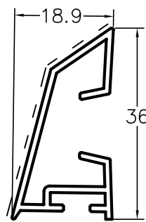
L50810 pingadeira
