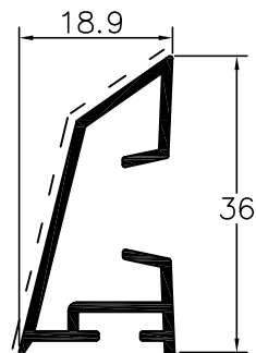
L50810 pingadeira
